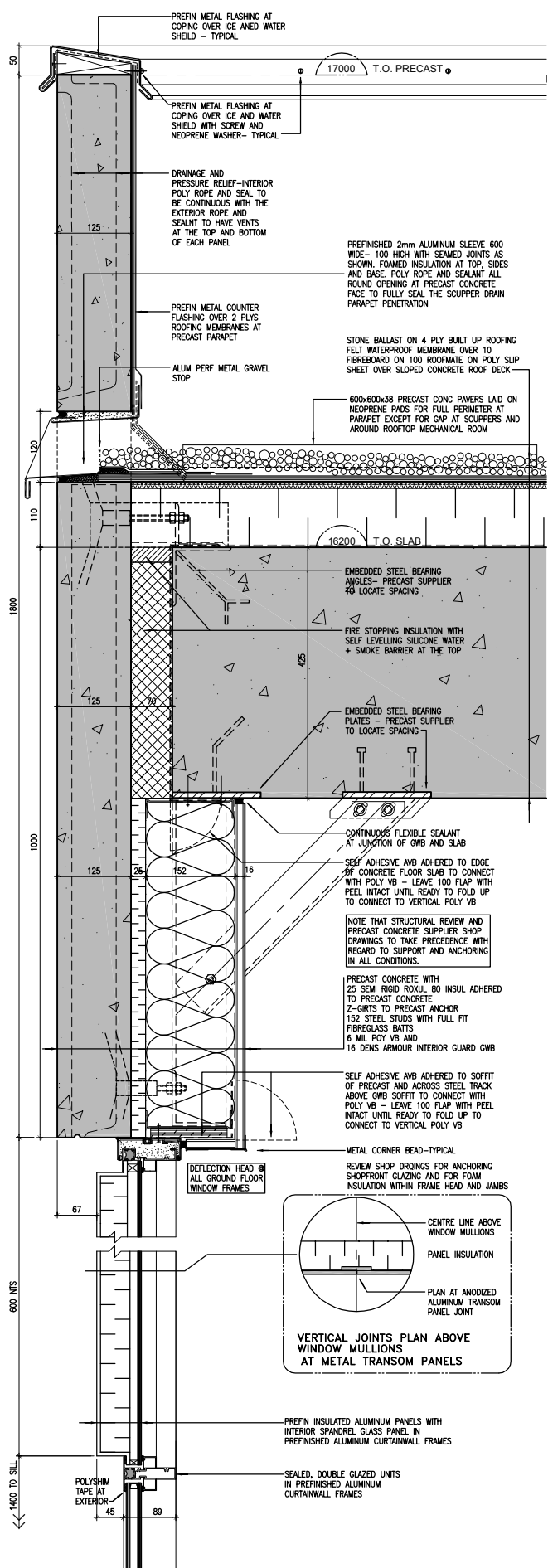
3 SECTION AT FOURTH FLOOR PARAPET A-801 SCALE: 1:5
