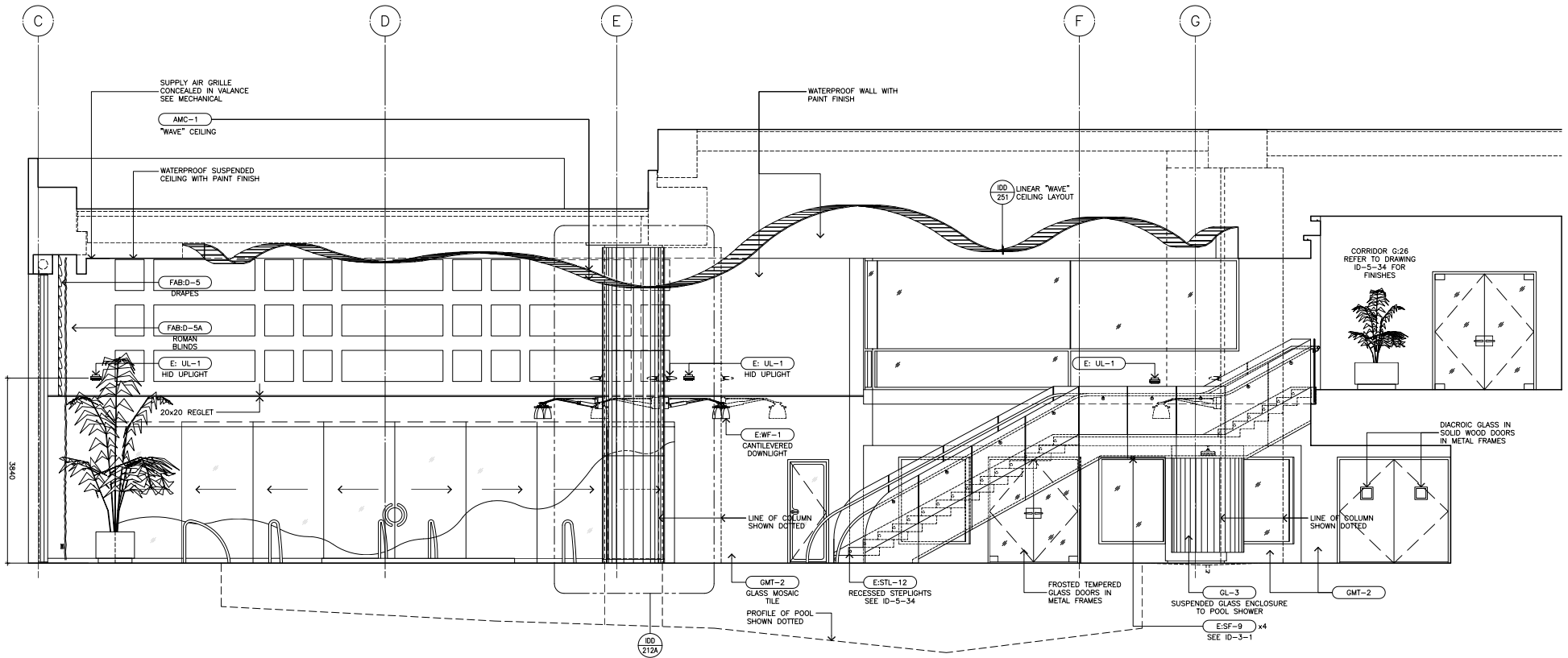
SWIMMING POOL DECK WEST INTERIOR ELEVATION SCALE 1:50
