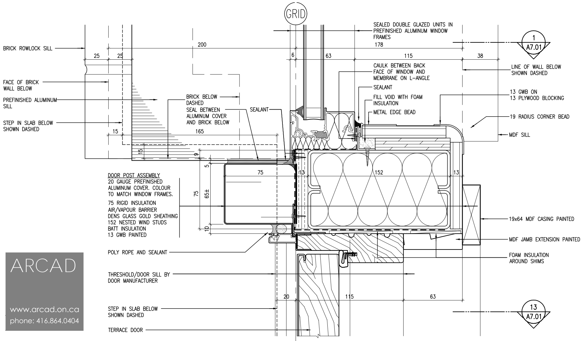
4 PLAN DETAIL TYPICAL PATIO DOOR AT WINDOW JAMB 1:2
